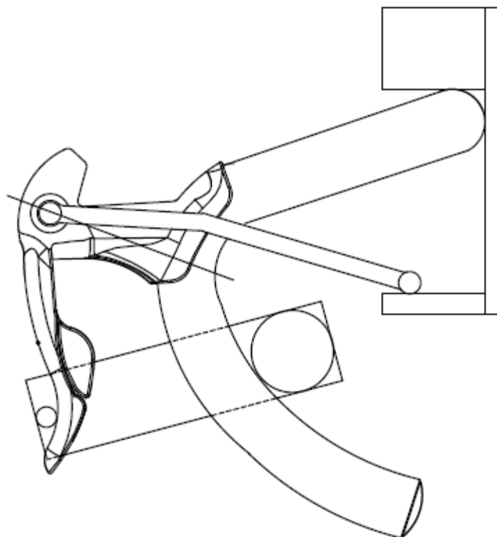
Figure 4 — Method of fitting the gauge to the brake lever and handlebar for type C
